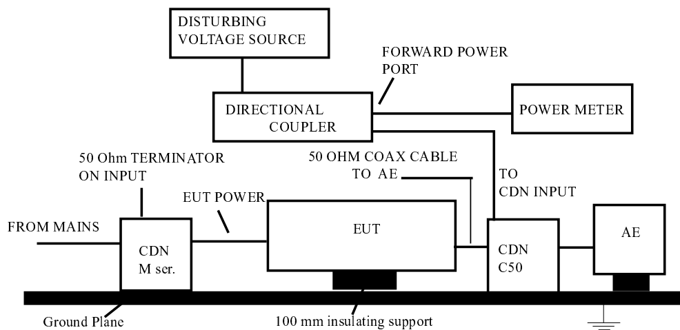
Figure 3-1 Conduced Immunity test setup using S series CDNs
