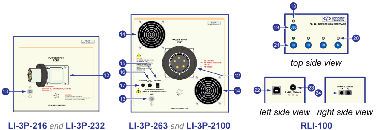
FIGURE 2 - Product Features – LISN Rear Panel & RLI-100
